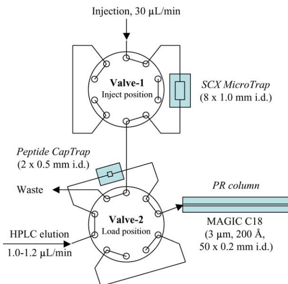
Fig. 1. Two-valve switching system configuration for two-dimensional peptide separation.
